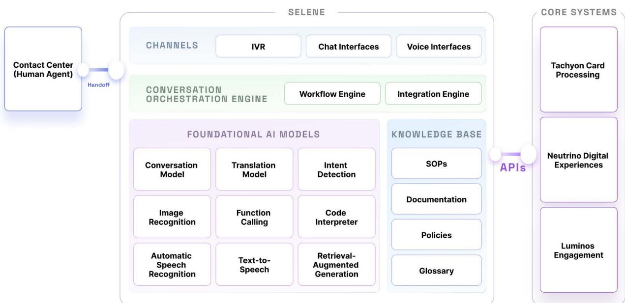
Image 3: Selene's 3-Layer Architecture
